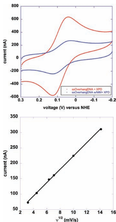
Figure 1. Electrochemistry of DNA-bound WT SaXPD. (Top) Cyclic voltammogram of SaXPD [ 120 \mu\text{M} ] on a well-matched DNA-modified electrode (red) and on DNA with a CA mismatch located near the gold surface as in Scheme 1 (blue) (Ag/AgCl reference electrodes, Pt auxiliary electrode, 50 \text{ mV/s} scan rate, NHE = normal hydrogen electrode). (Bottom) Plot of current versus v^{1/2} (square root of scan rate). The data indicate that our signal is obtained through a diffusion-limited process.
