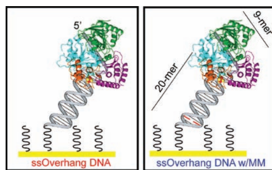
Scheme 1. Cartoon Schematic of Well-Matched DNA with a Nine-Nucleotide Single-Strand Overhang (Left) and DNA with a CA Mismatch shown in red (MM) (Right)
