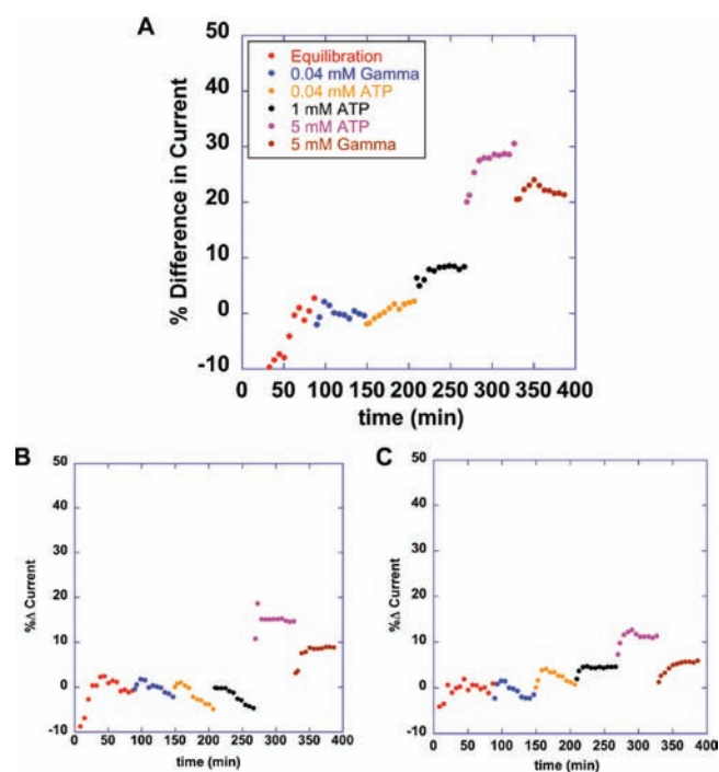
Figure 2. ATP-dependent electrochemistry of SaXPD on different DNA substrates. Time points shown are every 6 min (Ag/AgCl reference electrode, Pt auxiliary electrode, 50 \text{ mV/s} scan rate). Percent difference in current for SaXPD [ 9 \mu\text{M} ] on a 5'-ssDNA overhang (A), a 3'-ssDNA overhang (B), and fully duplexed DNA (C). The signal is seen to be ATP-dependent and sensitive to substrate. Note at the high-concentration addition [ 5 \text{ mM ATP-}\gamma\text{-S} ], some ATP still remains; once depleted, the signal levels off.
