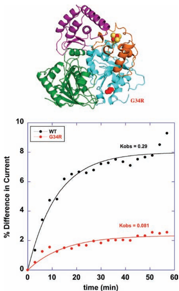
Figure 3. Electrochemical comparisons of SaXPD mutants after 5 mM ATP addition. (Top) Crystal structure of SaXPD with residues that were mutated shown in space filling model. Also shown in space-filling models is the [4Fe-4S] cluster. (Bottom) ATP-dependent CT of WT (black) and G34R (red). Observed initial rate constants (first 10 min) of 0.29 and 0.08 \text{min}^{-1} for WT and G34R.
